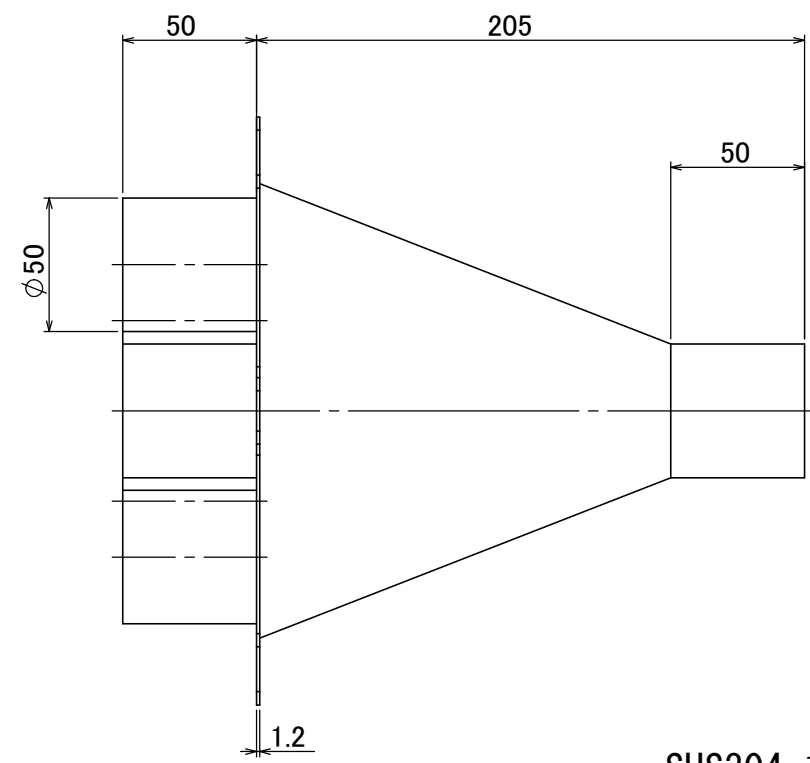
SUS304 1.2t 2" inlet-2"x5 outlet Manifold 2" (φ50inlet) 2"-5口 (φ50outlet) Manifold
